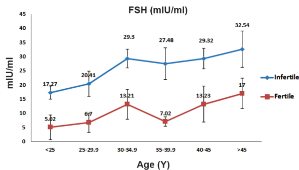
Fig.3: Mean ± standard follicle stimulating hormone (FSH) values for the reproductive age range in control and infertile group women.
